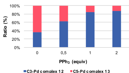
Figure 3. Effect of \text{PPh}_3 on the observed ratio of C3–Pd to C5–Pd complex. Conditions: \text{Pd}(\text{PPh}_3)_4 (10 mol %), \text{CuI} (1.0 equiv), \text{PPh}_3 , DMF (0.1 M), 23 °C.
