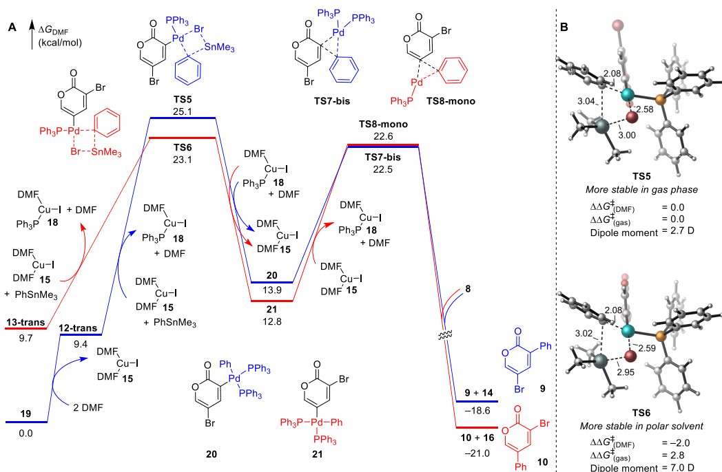
Figure 4. (A) Transmetalation and reductive elimination steps in the Pd-catalyzed Stille cross-coupling reaction of 3,5-dibromo-2-pyrone. The C3- and C5-selective pathways are shown in blue and in red, respectively. (B) Relative activation energies of transmetalation in an implicit solvent ( \Delta\Delta G_{\text{DMF}}^{\ddagger} ) and in the gas phase ( \Delta\Delta G_{\text{gas}}^{\ddagger} ). All energies in part A are with respect to 19 , two DMF molecules, and \text{PhSnMe}_3 . The energies in part B are with respect to TS5.
